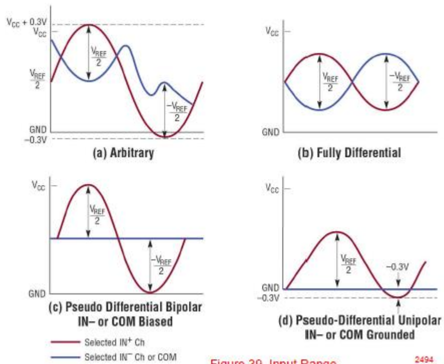
Figure 39. Input Range
