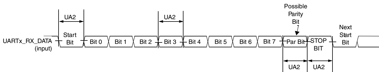
Figure 102. UART RS-232 Serial Mode Receive Timing Diagram
