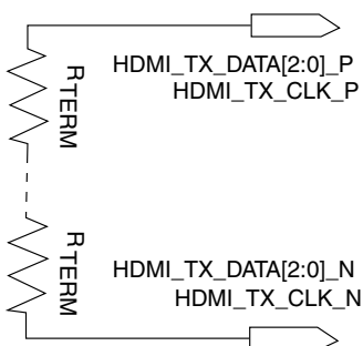
Figure 59. Source Termination
