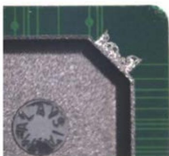
Visual appearance WITHOUT mousebite
