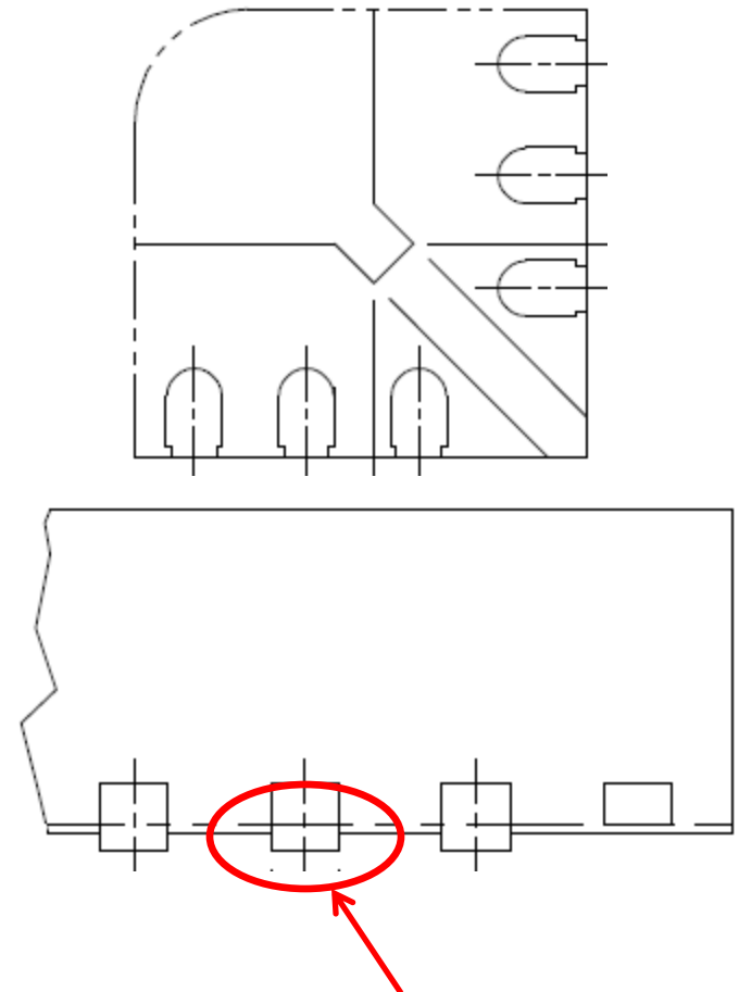
New Case drawing on Cu wire LF (E-type)
