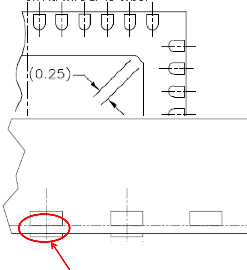
Original Case drawing on Au wire LF (S-type)
