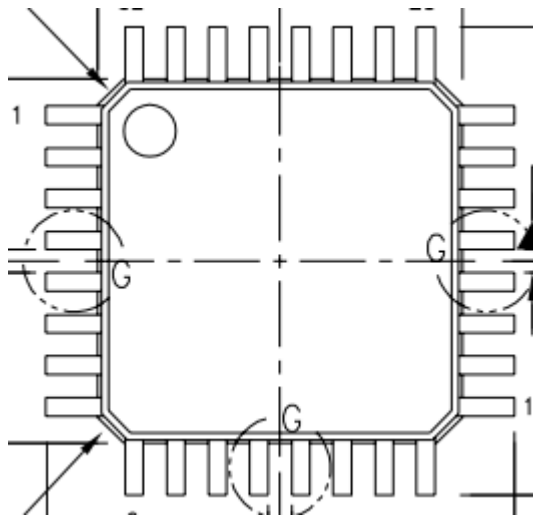
Figure 1. TJN Device
