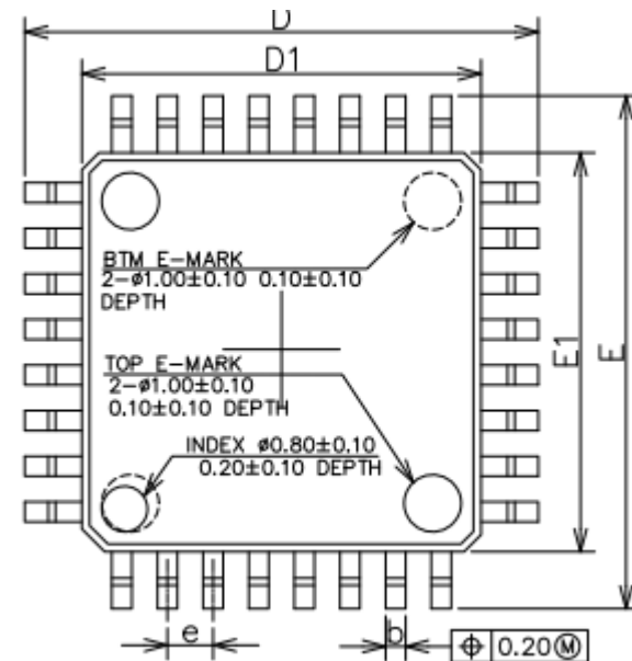
Figure 2. NFME Device
