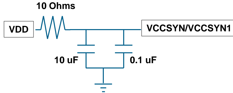
Figure 1-1 Original PLL Power Supply Filter Circuit for VCCSYN and VCCSYN1
