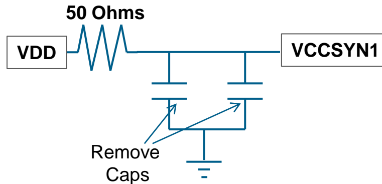
Figure 1-2 PLL Power Supply Filter Circuit Work Around
